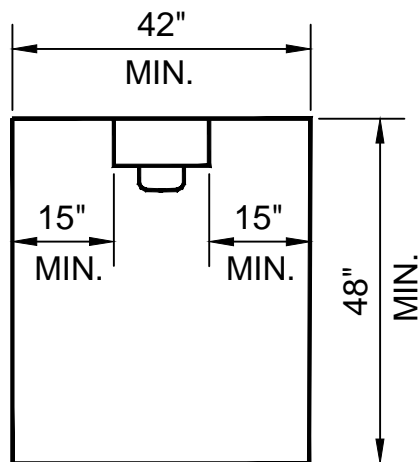
DECK PLAN (MINIMUM CLEARANCES)
