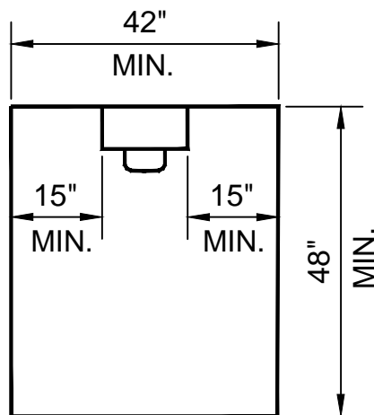
DECK PLAN (MINIMUM CLEARANCES)
